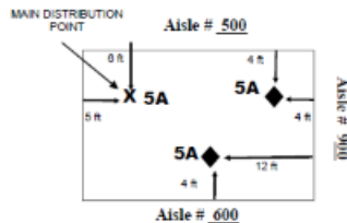
EXAMPLE-FLOOR POWER
